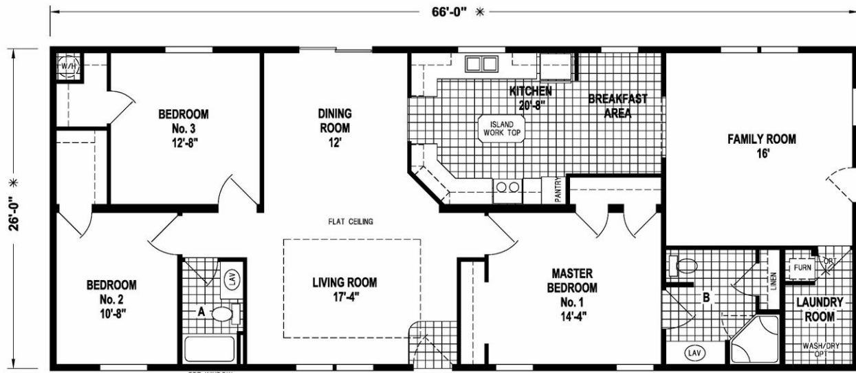
S1510Q-L1/6628 (1,716 SQ. FT.) 3BEDROOM - 2BATHS
